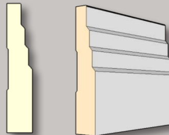
3 Step Skirting EDM 02 - 67x18 EDM 03 - 92x18 EDM 01 - 140x18
