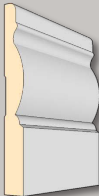
Talia Skirting EDM 2005 - 140x18
